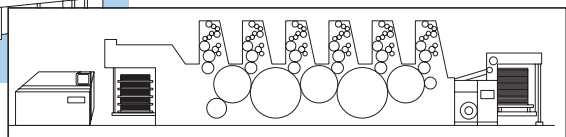
▼6-color machine
