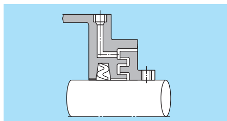
Fig. 8 Combination seal
