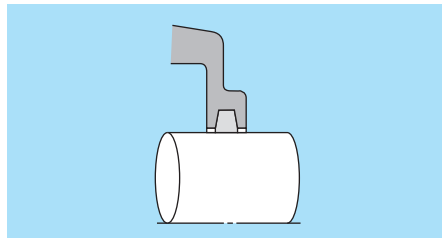
Fig. 4 Felt seal
