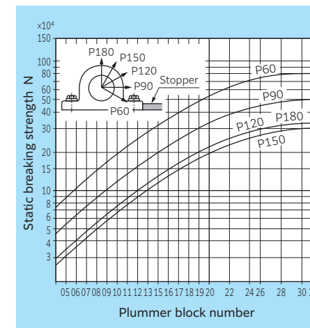
Fig. 10 Static breaking strength of SN6 (S6) series
