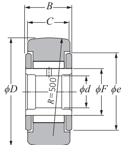
NATV type (Full complement roller type)
