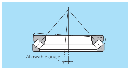
Fig. 2 Thrust spherical roller bearings
