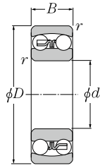
Cylindrical bore
